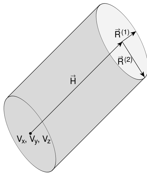
Fig. 8.5: Right Circular Elliptical Cylinder (REC)
