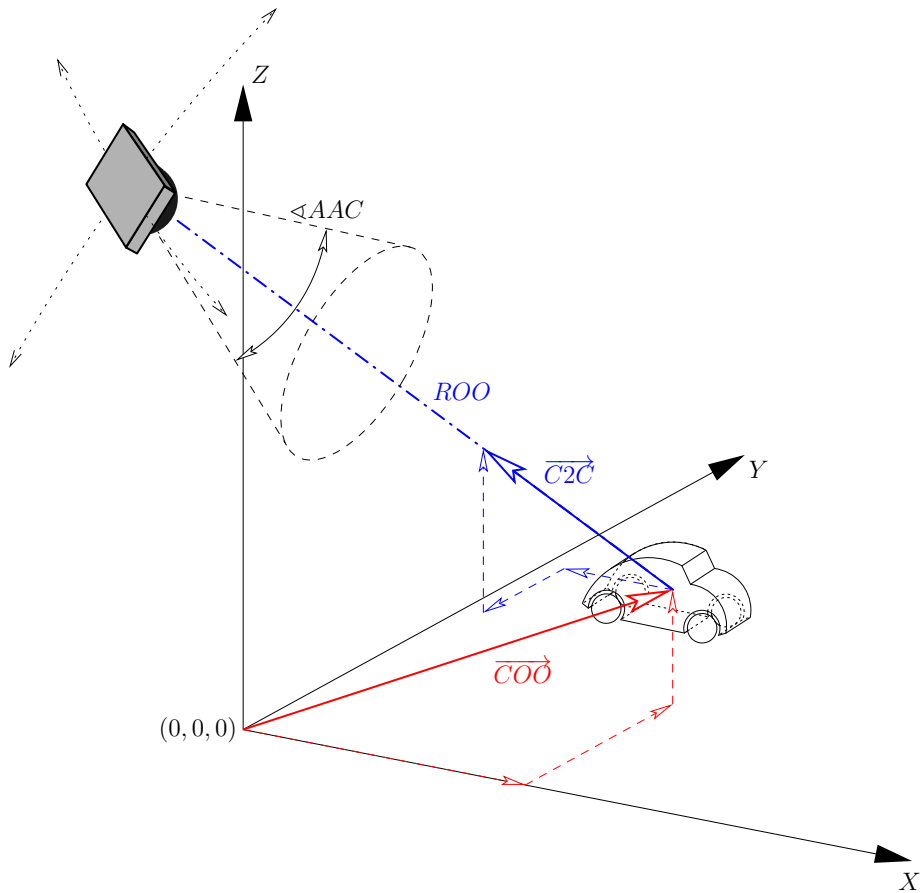
Figure 8: Camera and 3D object in the World System XYZ ; centre of orbit position vector \hat{C} , centre of orbit to camera direction vector \overrightarrow{C2C} , radius of orbit ROO , aperture angle of camera \sphericalangle AAC .
