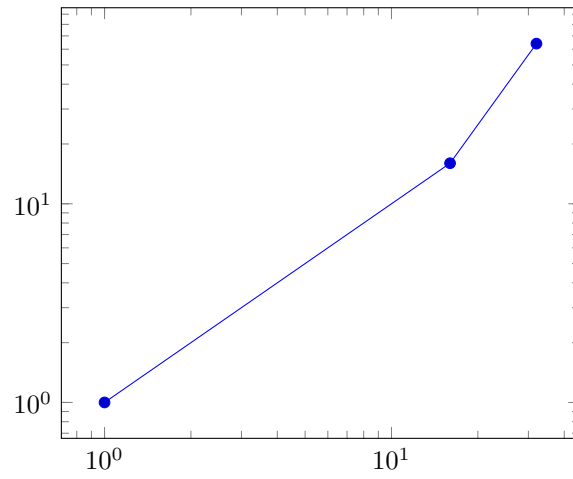
Figure 1: A small example
