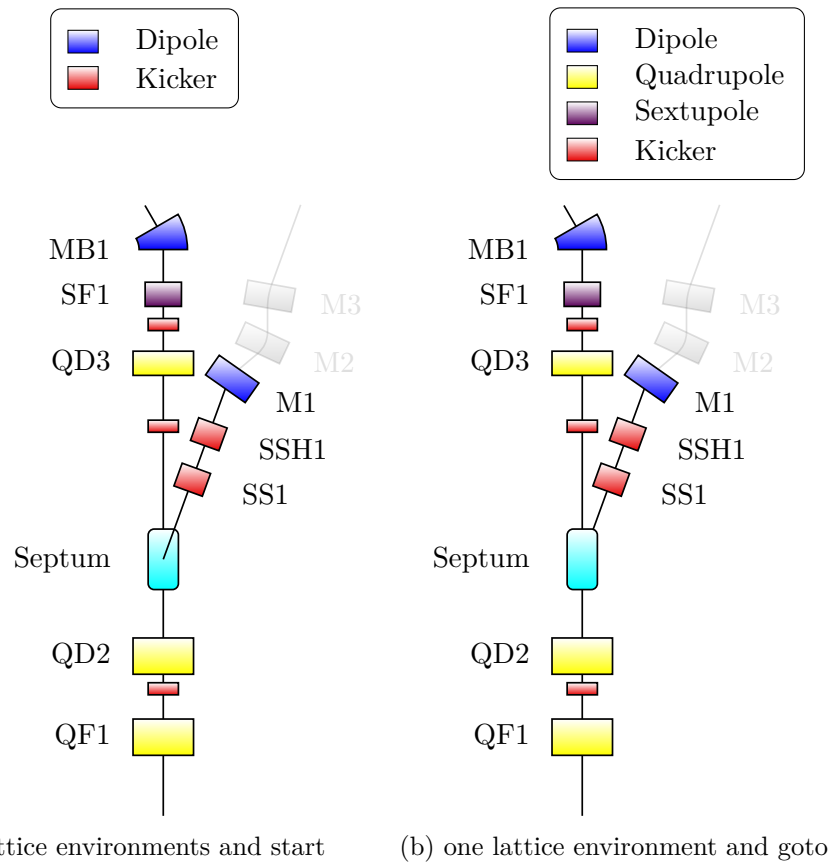
Figure 4: From example 3: Two ways to connect lattices
