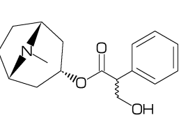
[75] Atoropin
