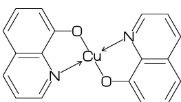
[12] Oxine-Copper
