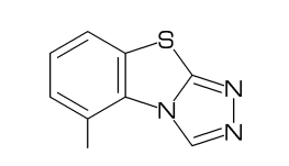
[32] Tricyclazole
