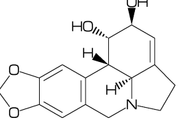
[50] Limonin
