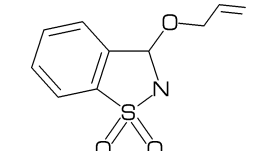
[34] Probenazole
