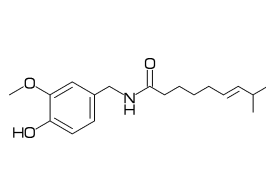
[73] Capsaicin
