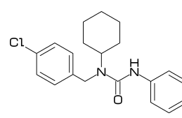
[24] Cyclosulfamuron
