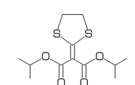
[10] Isoprothiolane
