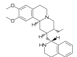
[52] Emetine
