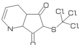
[13] Captan
