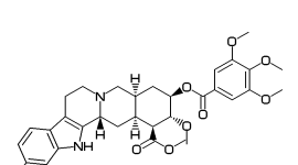
[65] Reserpine
