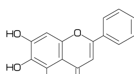
[64] Baicalein
