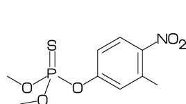
[6] Fenitrothion
