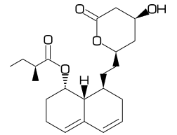
[75] Atoropin
