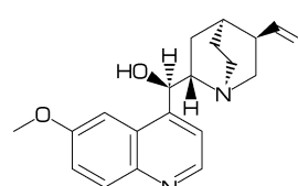
[74] Quinine
