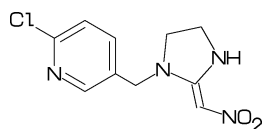
[7] Permethrin
