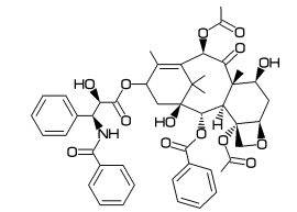
[74] Quinine
