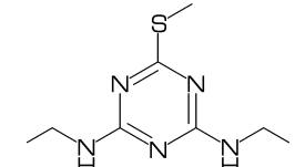
[35] Simetryn
