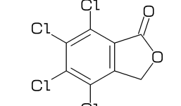
[33] Phthalide
