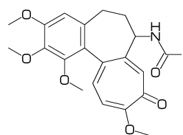
[53] Colchicine
