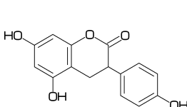
[62] Genistein
